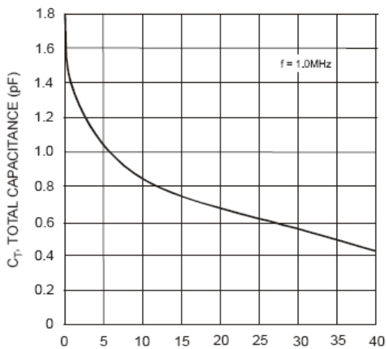
Fig. 3 Typical Capacitance
